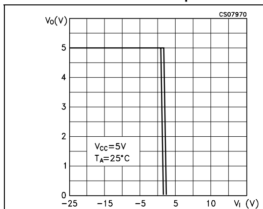
Figure 8. Voltage transfer characteristics for transmitter inputs
