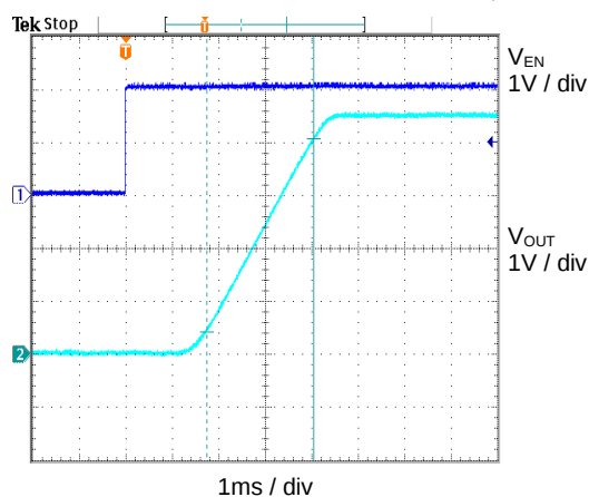
Turn-On Response ( V_{IN} = 4.5V , C_{OUT} = 100\mu F , R_L = 150\Omega )
