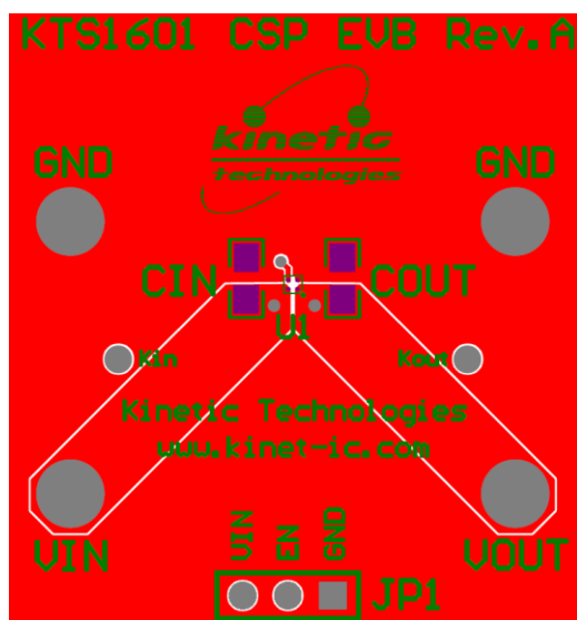
Figure 2. KTS1601 Evalauation Board Layout (TOP Layer)
