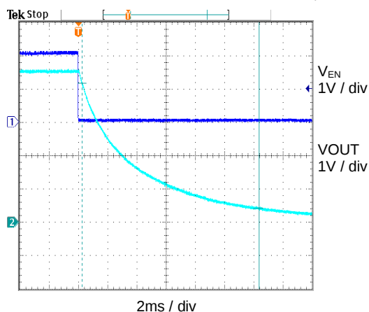
Turn-Off Response ( V_{IN} = 4.5V , C_{OUT} = 100\mu F , R_L = 150\Omega )
