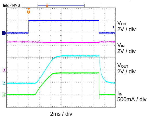
Turn-On & Turn-Off Response ( V_{IN} = 4.5V , C_{IN} = 10\mu F , C_{OUT} = 100\mu F , R_L = 5\Omega )
