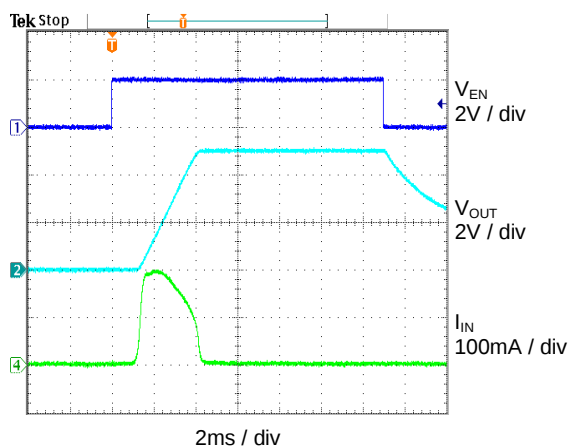
In-rush Current Waveform ( V_{IN} = 5.0V , C_{IN} = 10\mu F , C_{OUT} = 100\mu F , R_L = \text{Open} )
