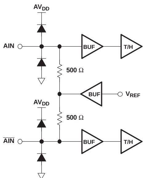
Figure 31. Analog Input
