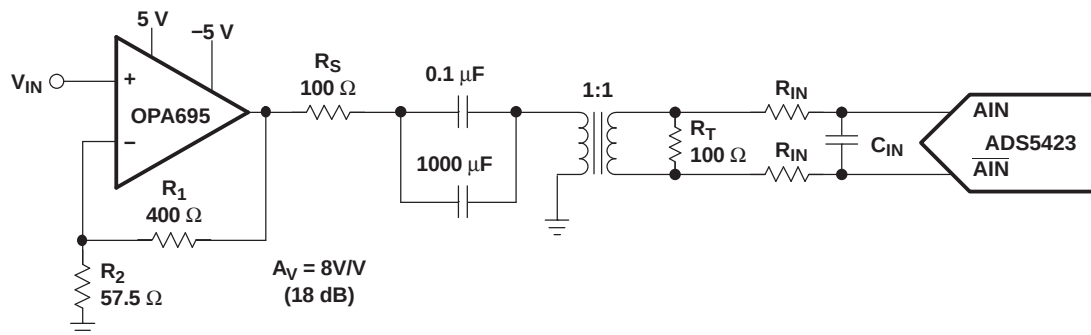
Figure 38. Using the OPA695 With the ADS5423
