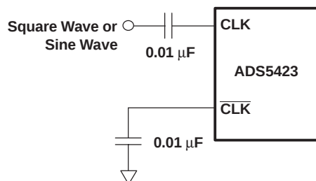
Figure 42. Single-Ended Clock
