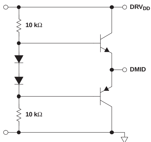
Figure 36. DMID Generation
