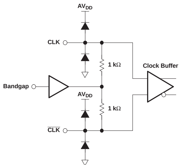
Figure 33. Clock Input
