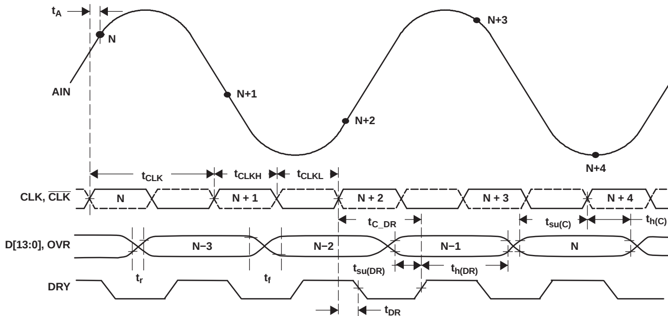
Figure 2. Timing Diagram
