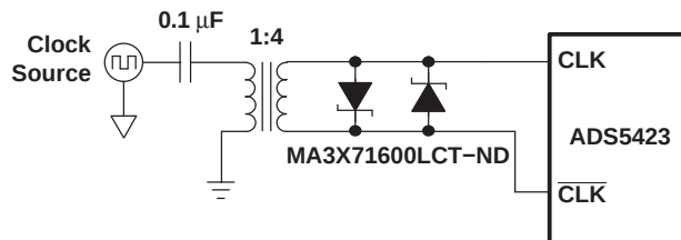
Figure 43. Differential Clock
