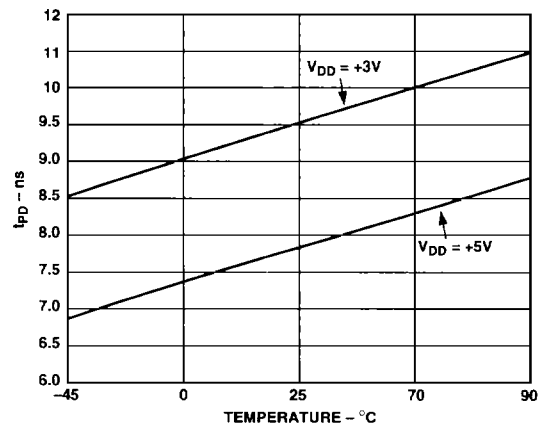
Figure 11. t_{PD} vs. Temperature/Supply ( V_{DD} = +3V/+5V )
