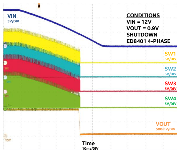
Shutdown with VIN at No Load (4-Phase)
