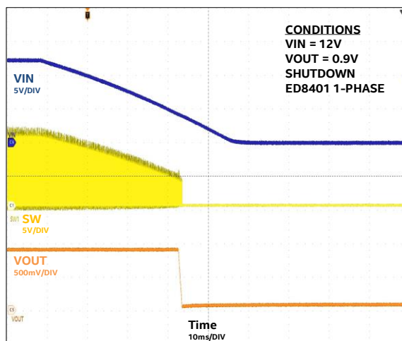
Shutdown with VIN at No Load (1-Phase)
