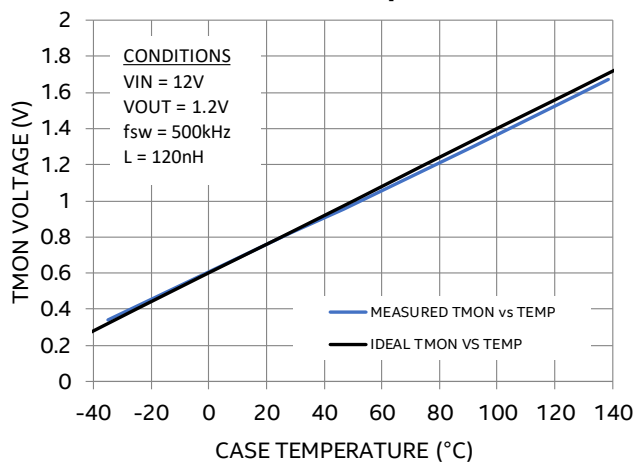
TMON vs. Temperature
