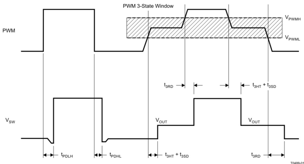
Figure 8: PWM Timing Diagram
