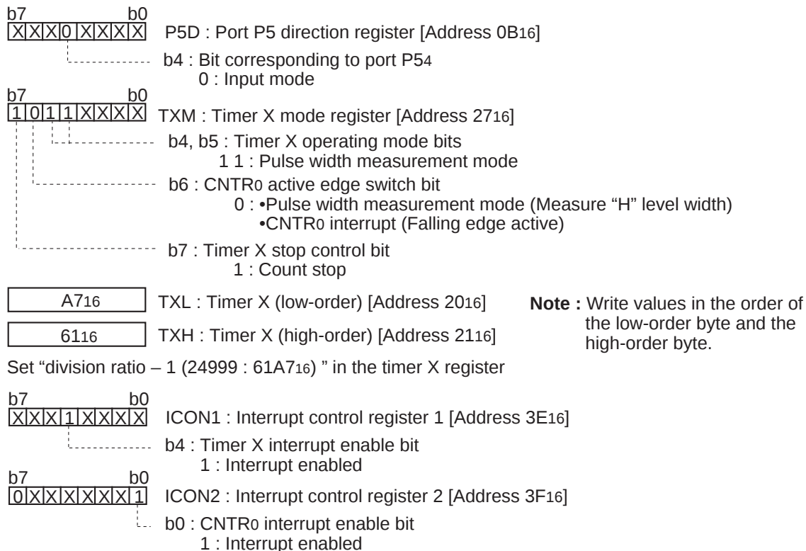
Fig. 2.3.36 Setting of related registers
