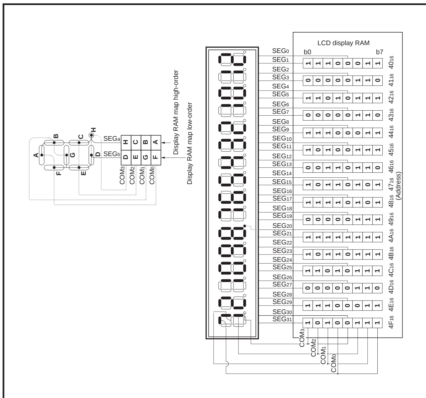
Fig. 2.7.9 8-segment LCD panel display pattern example when duty ratio number is 4
