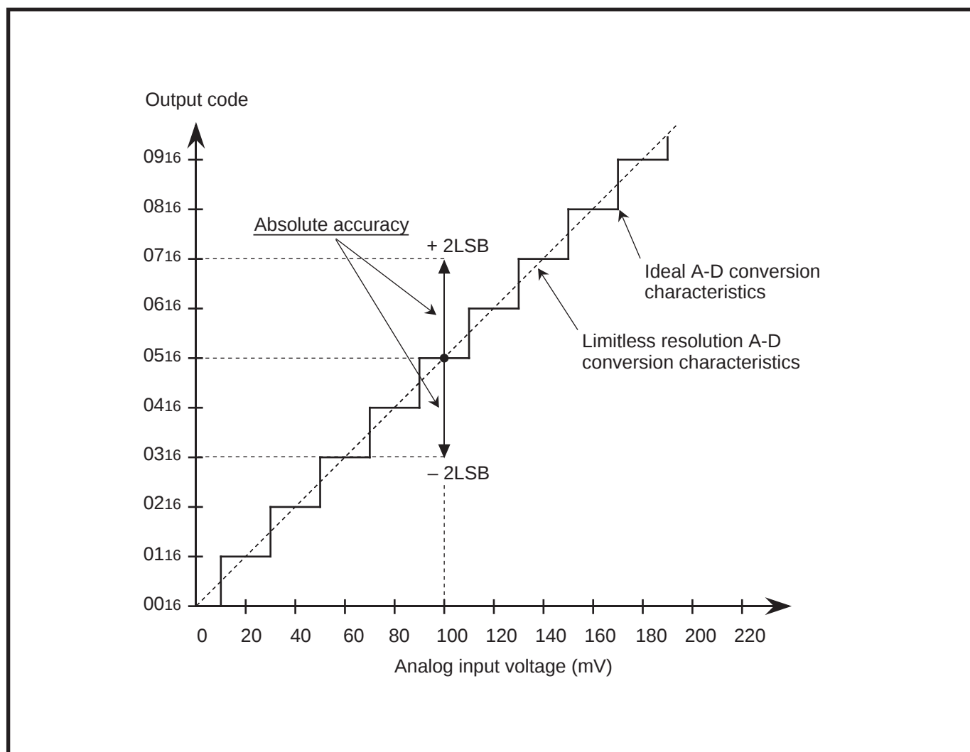
Fig. 2.6.11 Absolute accuracy of A-D converter
