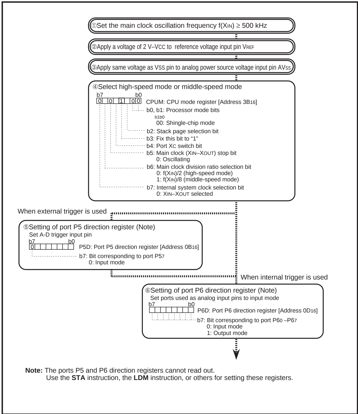
Fig. 2.6.13 Operating conditions for using A-D converter
