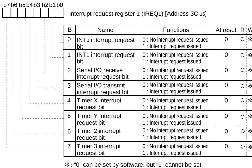
Fig. 3.3.17 Structure of interrupt request register 1
