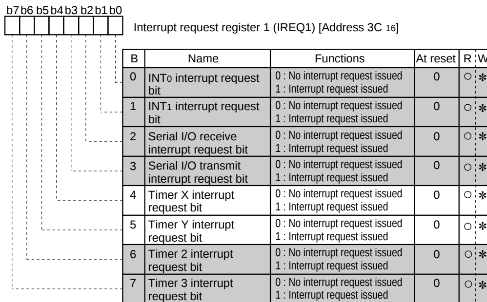
Interrupt request register 1
