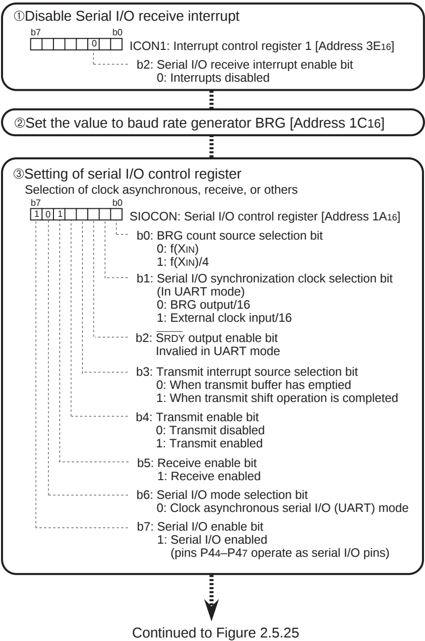
Fig. 2.5.24 Receiving method in UART mode (1)
