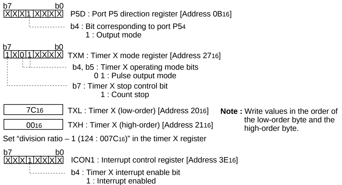
Fig. 2.3.33 Setting of related registers
