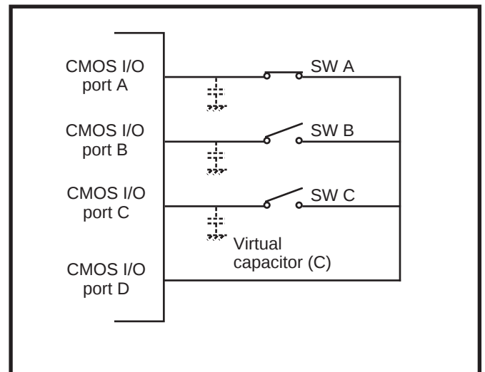
Fig. 2.1.10 Connection example 2 for key input
