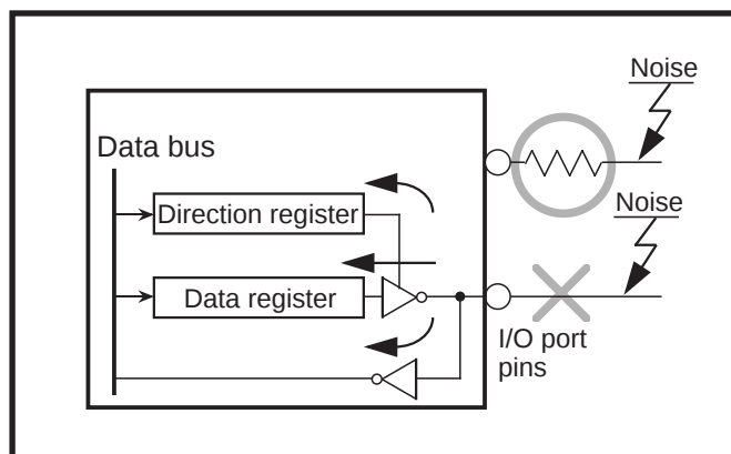
Fig. 3.2.9 Setup for I/O ports
