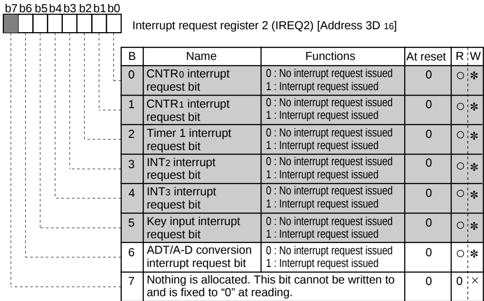
Interrupt request register 2
