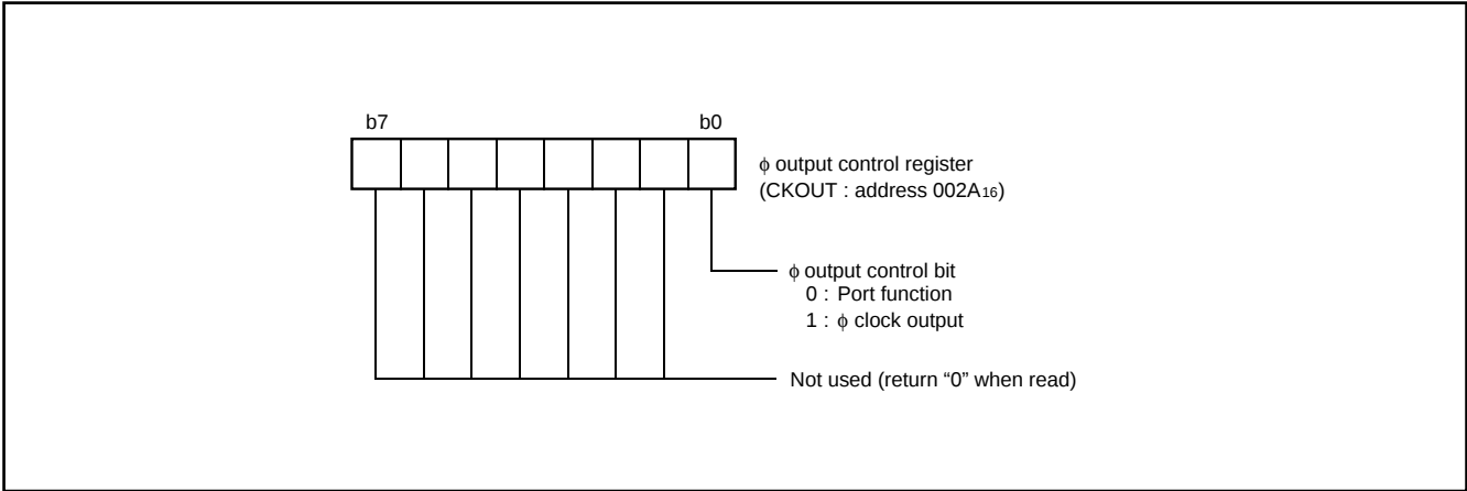
Fig. 34 Structure of \phi output control register
