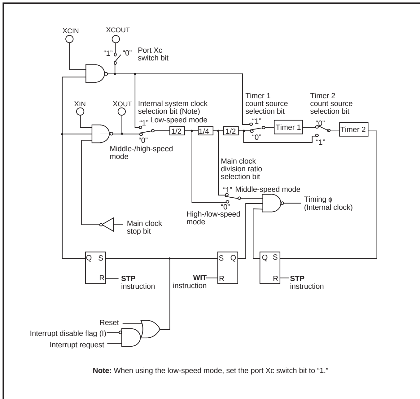
Fig. 2.10.3 Clock generating circuit block diagram
