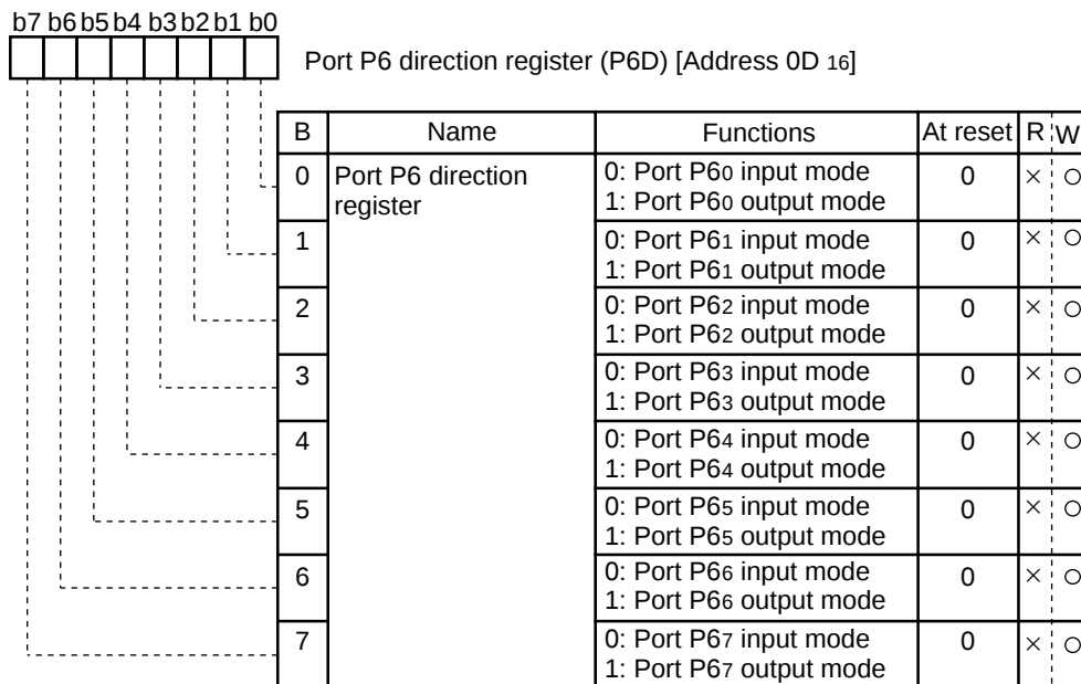
Port P6 direction register
