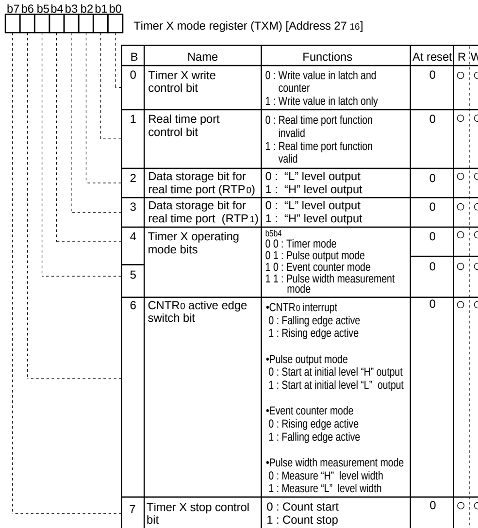
Timer X mode register
