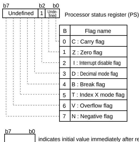
Processor status register
