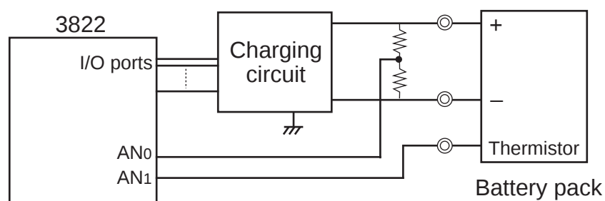
Fig. 2.6.18 Example of peripheral circuit
