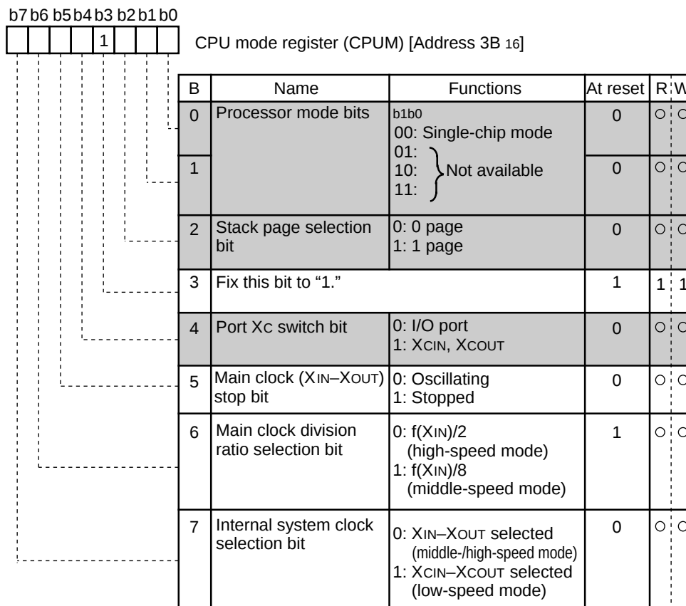
CPU mode register
