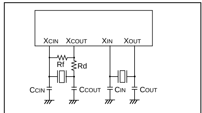
Fig. 38 Ceramic resonator circuit
