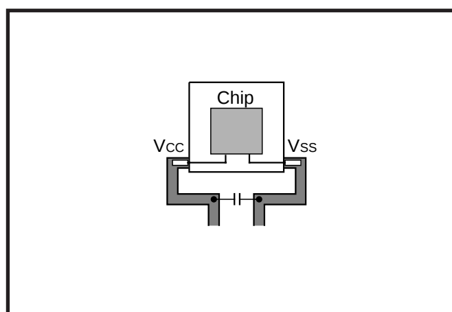
Fig. 3.2.4 Bypass capacitor across the Vss line and the Vcc line
