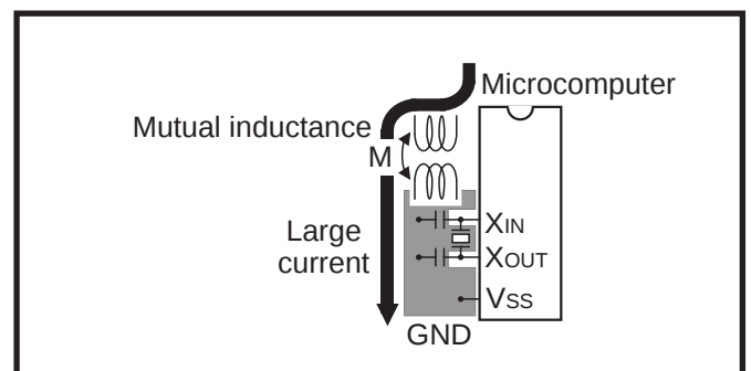
Fig. 3.2.6 Wiring for a large current signal line
