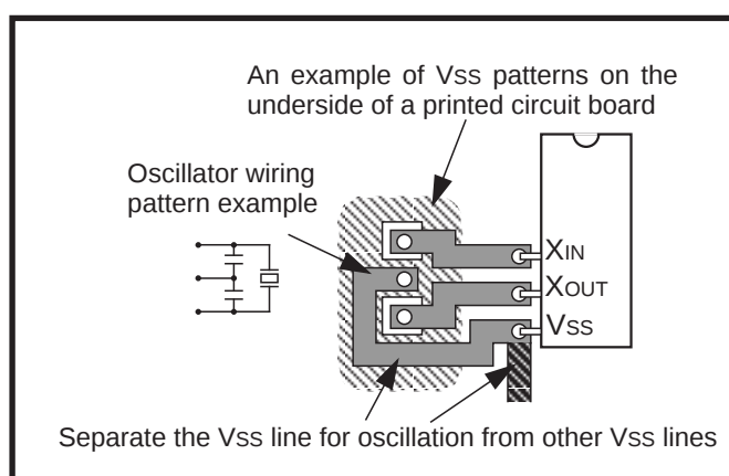
Fig. 3.2.8 Vss pattern on the underside of an oscillator
