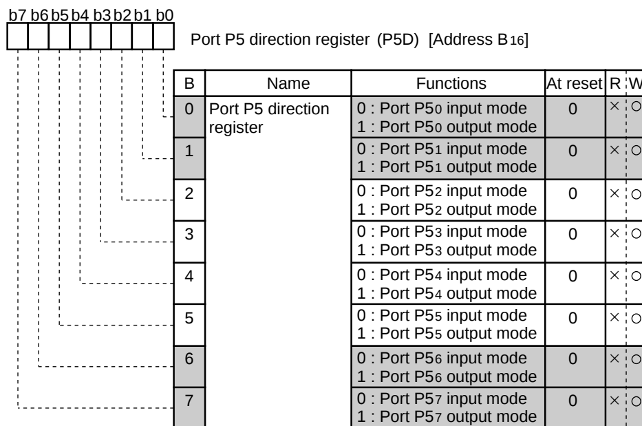
Port P5 direction register
