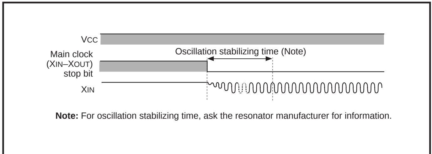
Fig. 2.10.7 Oscillation stabilizing time at reoscillation of X_{IN}
