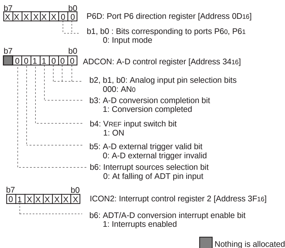
Fig. 2.6.19 Setting of related registers
