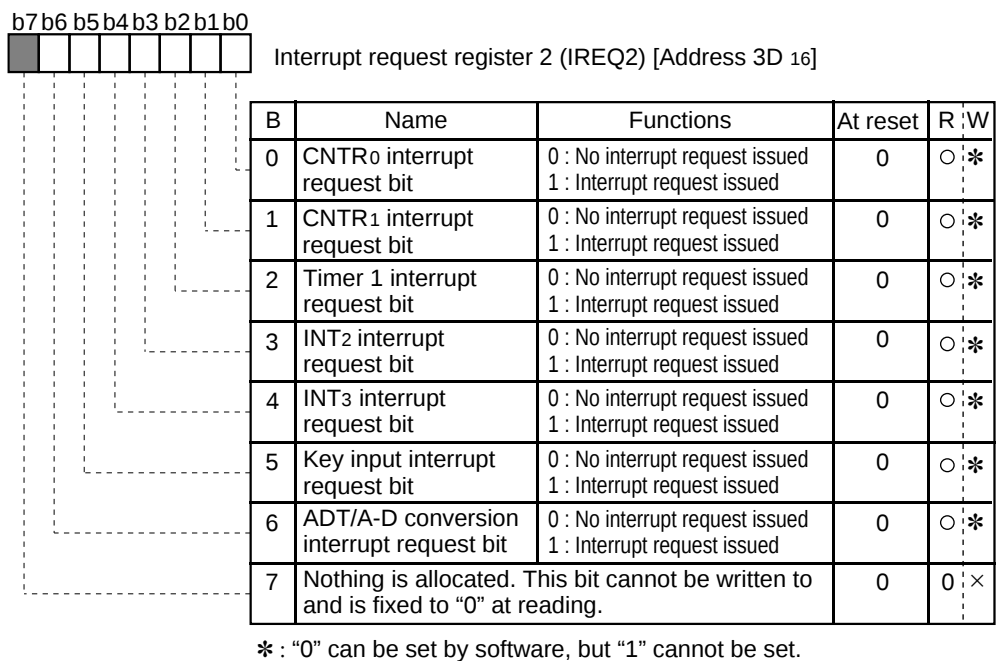
Fig. 3.3.18 Structure of interrupt request register 2
