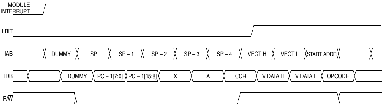
Figure 9-8. Interrupt Entry
