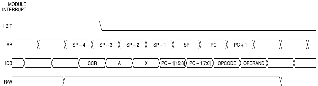
Figure 9-9. Interrupt Recovery
