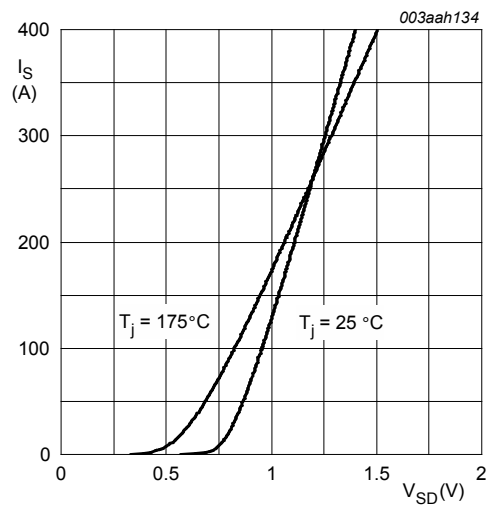
Fig. 16. Source (diode forward) current as a function of source-drain (diode forward) voltage; typical values V_{GS} = 0\text{V}
