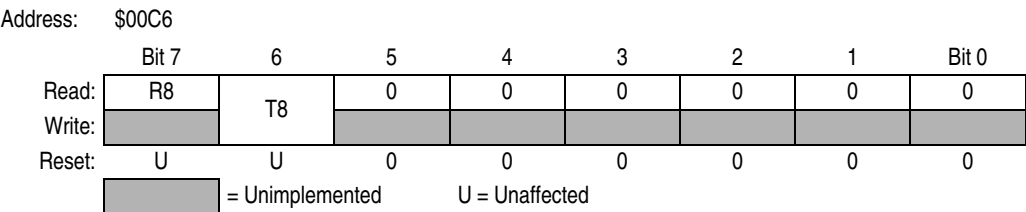
Figure 14-9. SCI Data Register High (SC0DRH)
