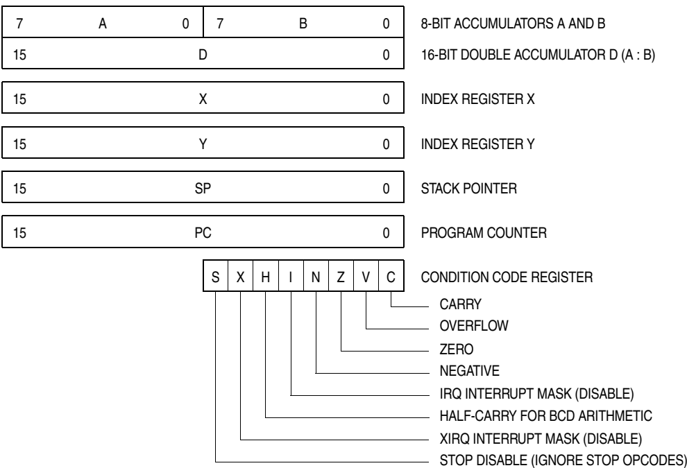
Figure 3-1. Programming Model
