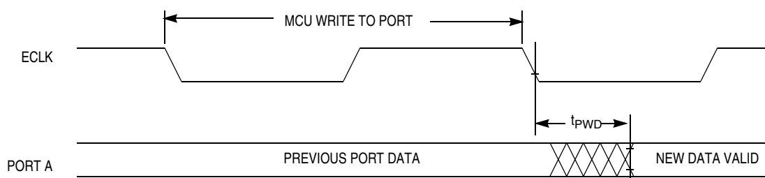
Figure 19-11. Port Write Timing Diagram
