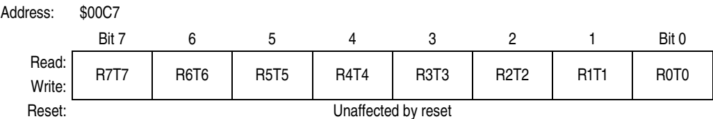
Figure 14-10. SCI Data Register Low (SC0DRL)
