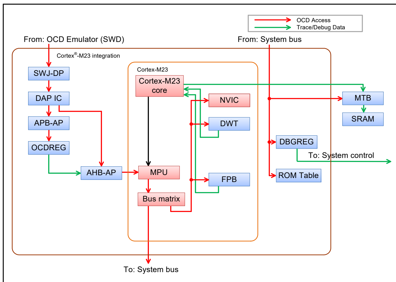
Figure 2.1 Cortex-M23 CPU block diagram
