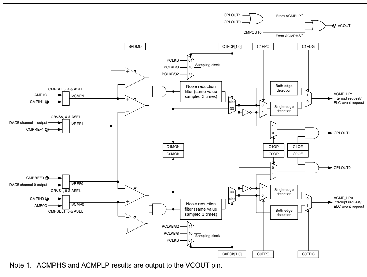
Figure 39.2 ACMLP block diagram when window function is enabled in window function mode
