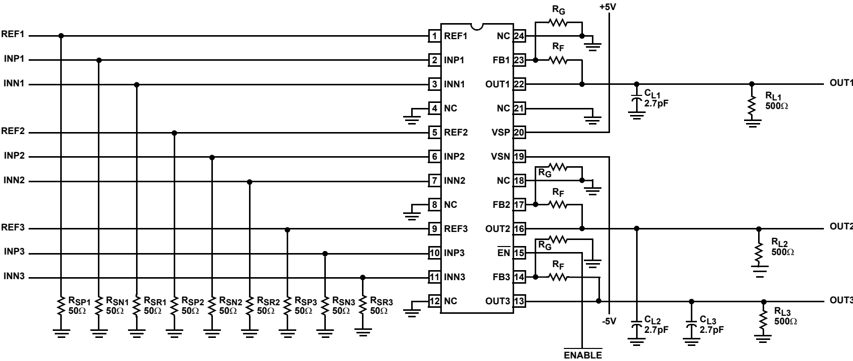
FIGURE 2. EL5375
