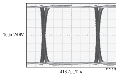
CMLOUT Eye Diagram 400Mbps
