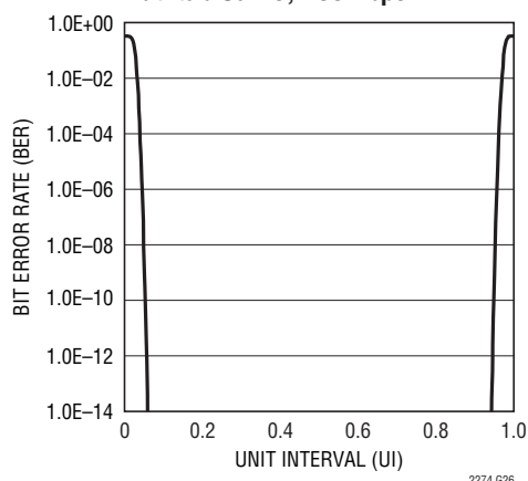
CMLOUT Dual-Dirac BER Bathhtub Curve, 400Mbps
