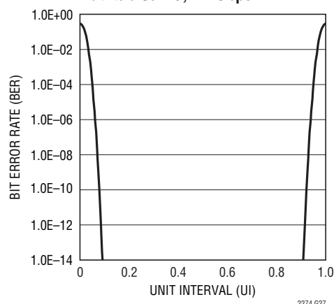
CMLOUT Dual-Dirac BER Bathhtub Curve, 1.2Gbps
