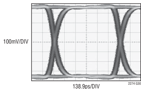
CMLOUT Eye Diagram 1.2Gbps
