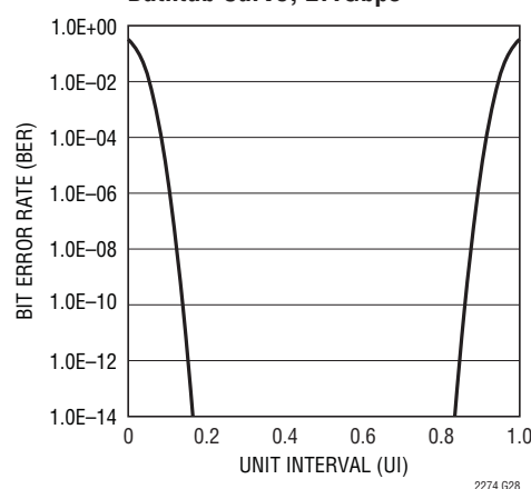
CMLOUT Dual-Dirac BER Bathhtub Curve, 2.1Gbps
