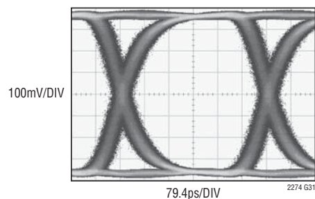
CMLOUT Eye Diagram 2.1Gbps
