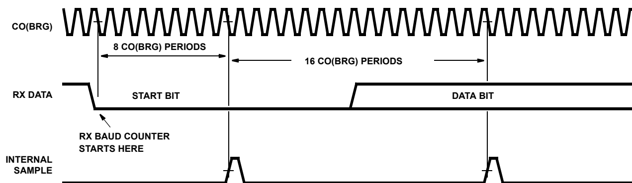
FIGURE 17. RECEIVER DATA
