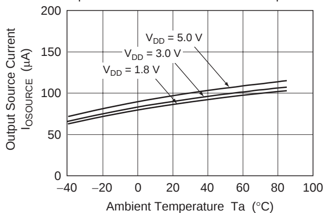
Figure 3-5. HA1630D03 Output Source Current vs. Ambient Temperature
