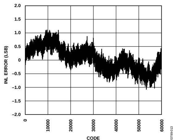
Figure 11. AD7386 Integral Nonlinearity (INL) Error
