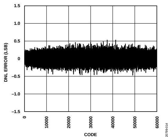
Figure 12. AD7386 Differential Nonlinearity (DNL) Error
