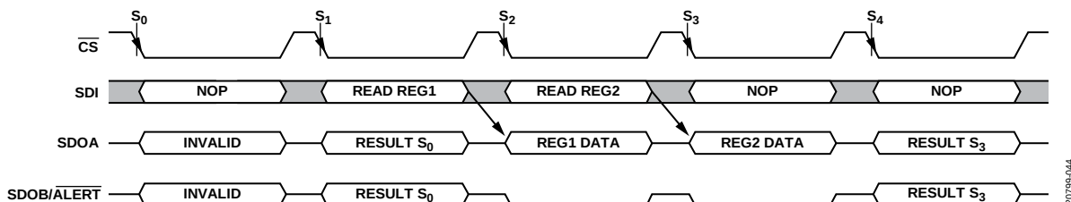
Figure 45. Register Read
