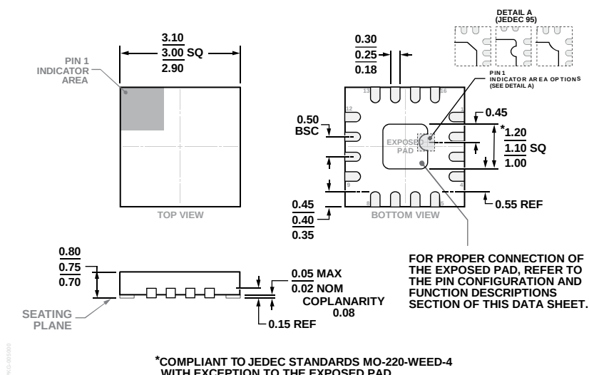
Figure 48. 16-Lead Lead Frame Chip Scale Package [LFCSP] 3 mm × 3 mm Body and 0.75 mm Package Height (CP-16-45)
