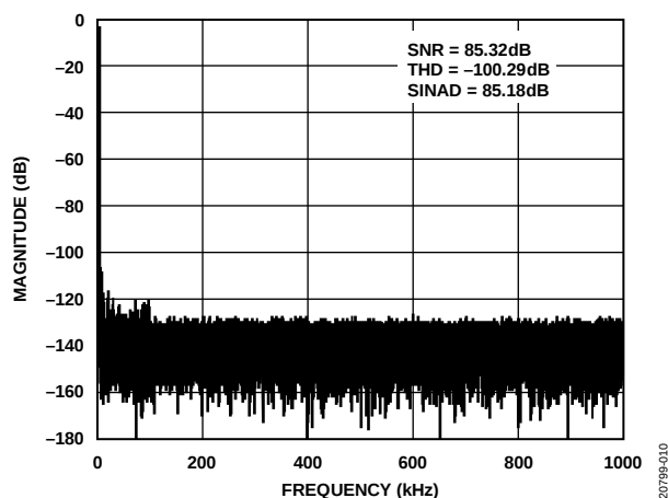
Figure 8. AD7386 Fast Fourier Transform (FFT), V_{REF} = 2.5 V Internal
