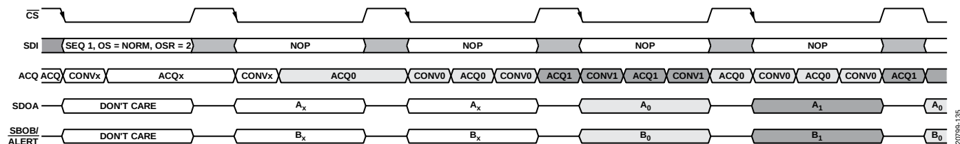
Figure 35. Normal Average Oversampling in Sequencer Mode
