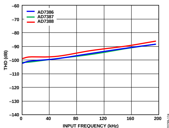
Figure 24. THD vs. Input Frequency
