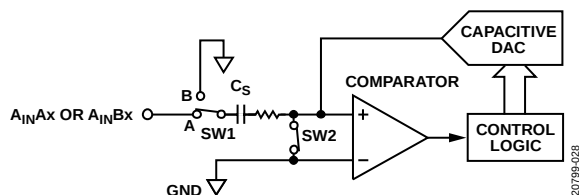
Figure 26. ADC Acquisition Phase
