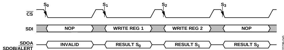
Figure 46. Register Write
