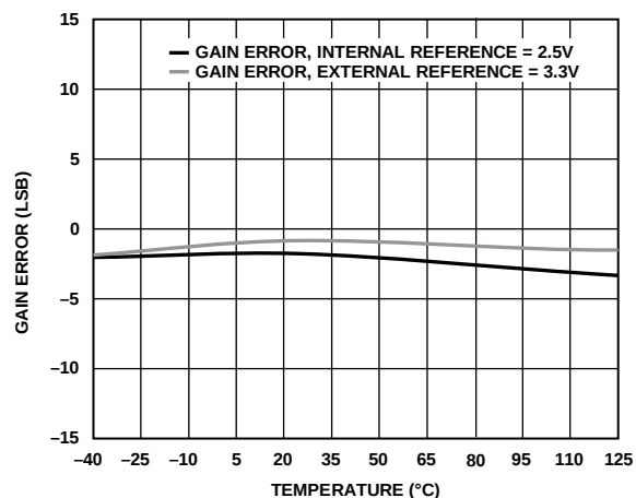
Figure 15. AD7386 Gain Error vs. Temperature
