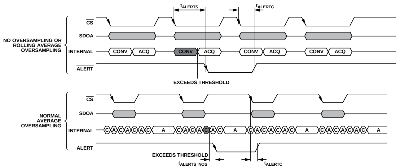
Figure 38. Alert Operation
