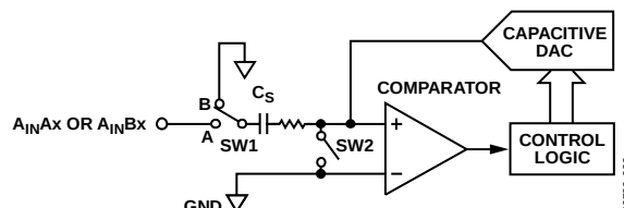
Figure 27. ADC Conversion Phase
