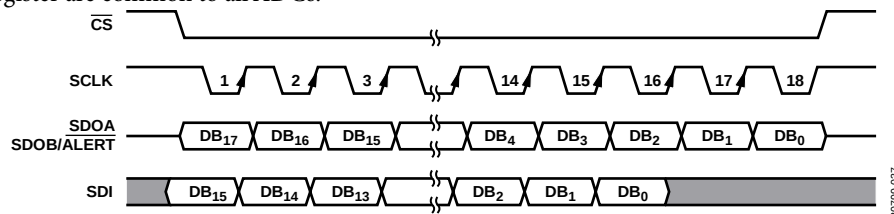
Figure 37. Resolution Boost
