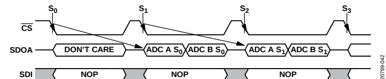
Figure 43. Read Conversion Results for 1-Wire Mode
