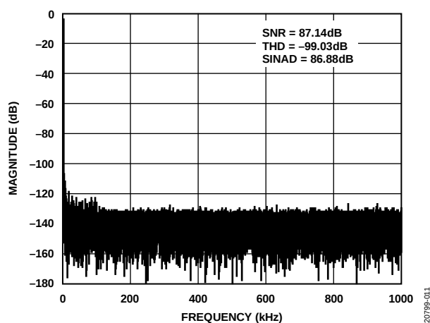
Figure 9. AD7386 FFT, V_{REF} = 3.3 V External
