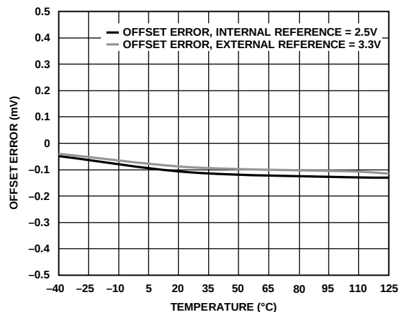
Figure 14. AD7386 Offset Error vs. Temperature
