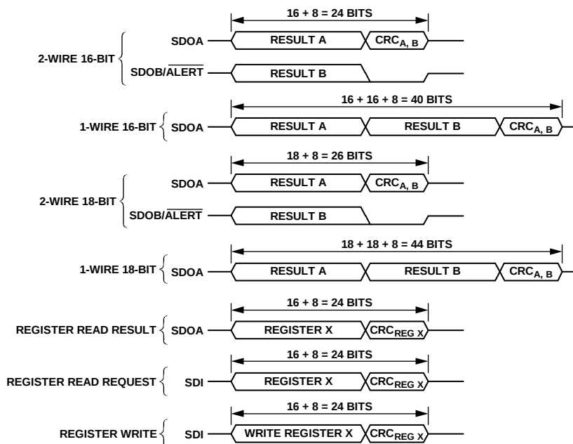
Figure 47. CRC Operation
