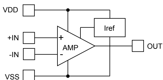
BD7281YG-C
