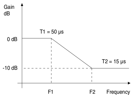
Figure 15. De-emphasis Curve
