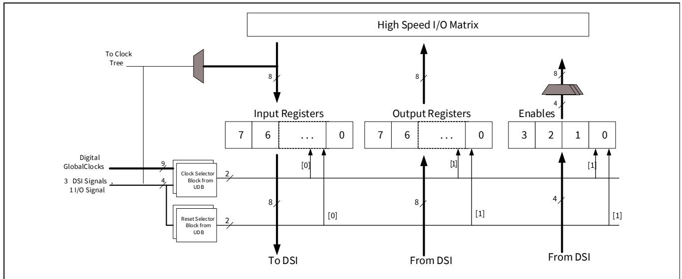
Figure 5 Port interface
