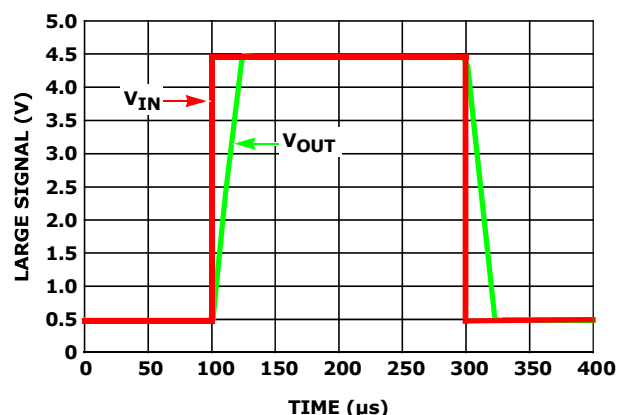
FIGURE 54. SIMULATED LARGE SIGNAL STEP RESPONSE (4V)
