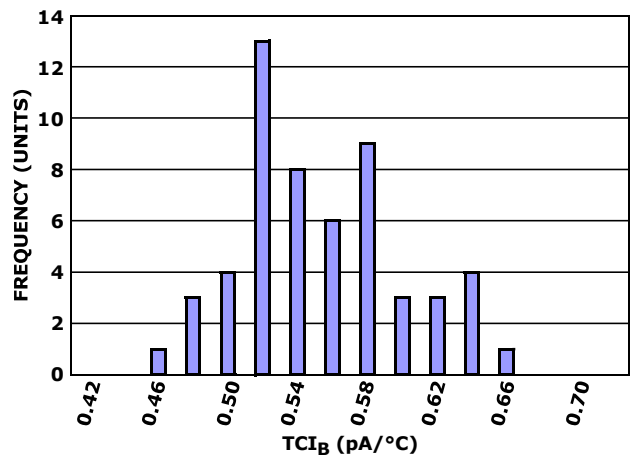
FIGURE 35. TCI_b HISTOGRAM
