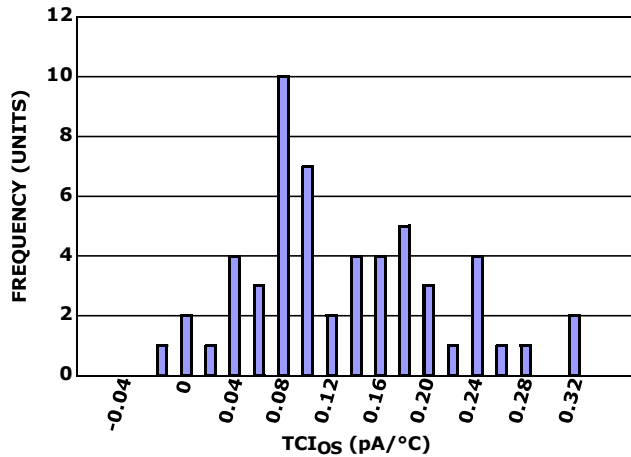
FIGURE 34. TCI_{0S} HISTOGRAM
