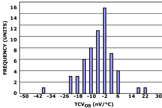
FIGURE 36. TCV_{OS} HISTOGRAM
