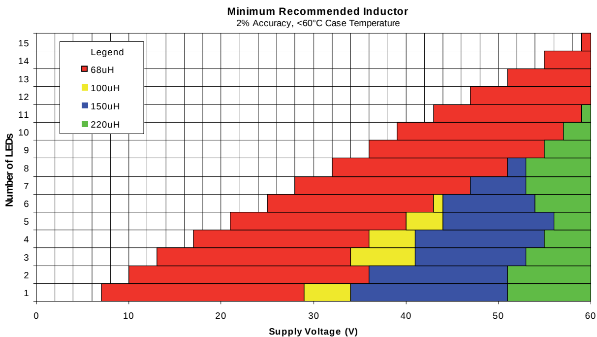
Figure 3. ZXLD1366Q Minimum Recommended Inductor (TSOT25)
