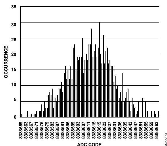
Figure 9. Histogram (Voltage Input, Output Data Rate = 2.5 kSPS)
