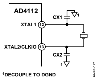
Figure 40. External Crystal Connections
