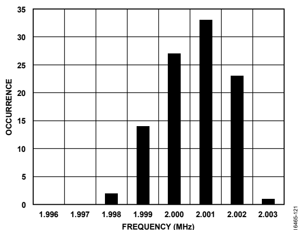
Figure 21. Internal Oscillator Frequency/Accuracy Distribution Histogram
