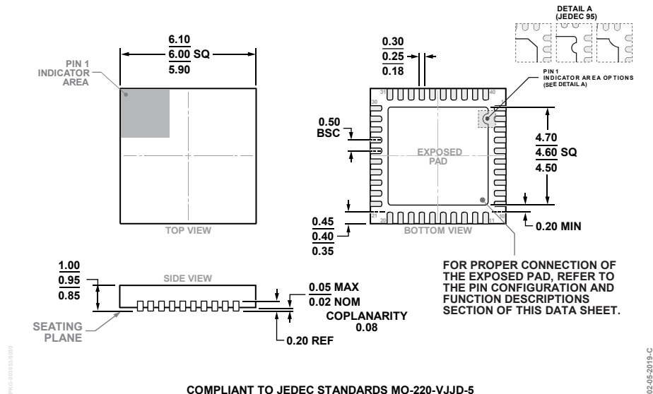
Figure 59. 40-Lead Lead Frame Chip Scale Package [LFCSP] 6 mm × 6 mm Body and 0.95 mm Package Height (CP-40-15)
