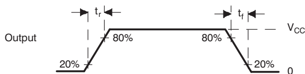
Figure 11. CMOS-Level Outputs
