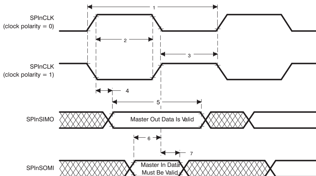
Figure 13. SPI Master Mode External Timing (CLOCK PHASE = 0)
