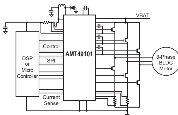
Figure 1: Typical Application
