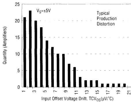
EL5410C Input Offset Voltage Drift
