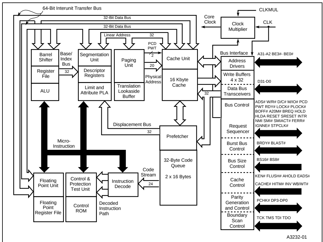
Figure 1. Embedded Write-Back Enhanced Intel® ID4™ Processor Block Diagram
