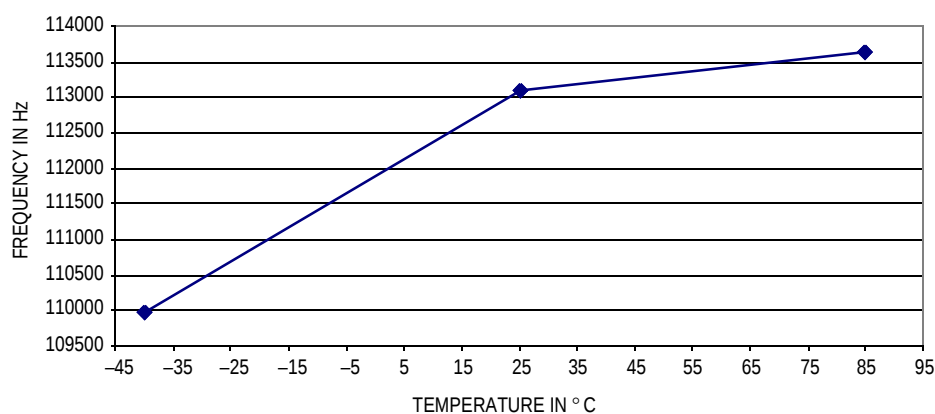
Figure 15-8. Typical 100 kHz External Low-Power Oscillator Frequency
