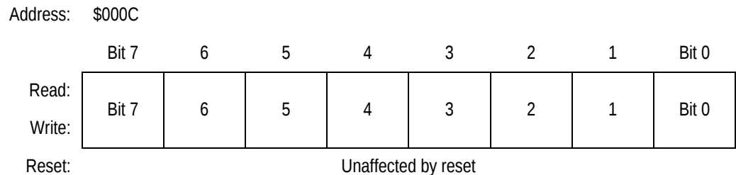
Figure 9-6. SIOP Data Register (SDR)
