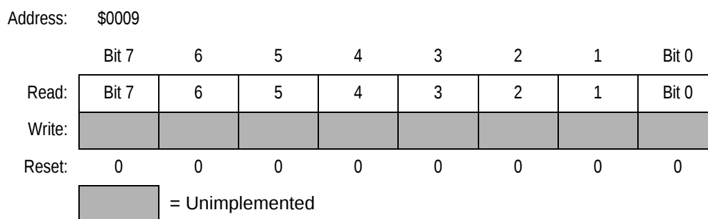
Figure 10-3. Core Timer Counter Register (CTCR)
