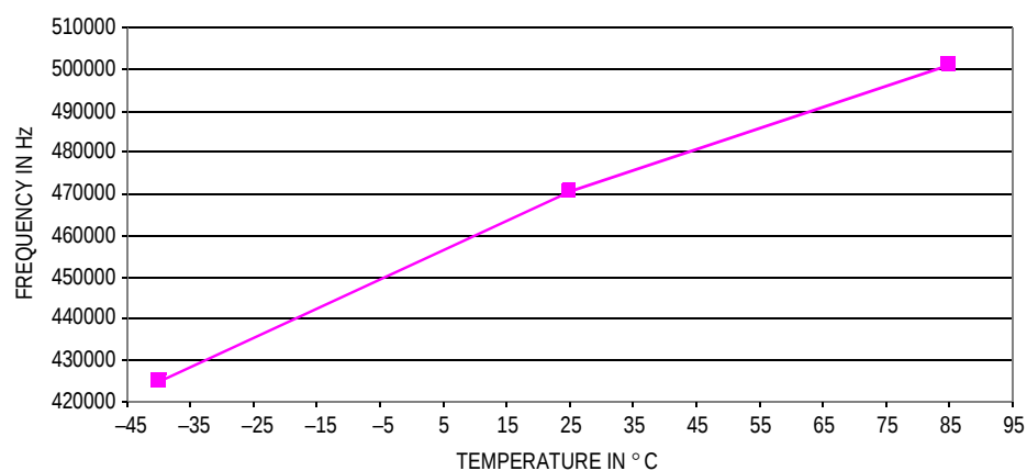
Figure 15-7. Typical 500 kHz External Low-Power Oscillator Frequency
