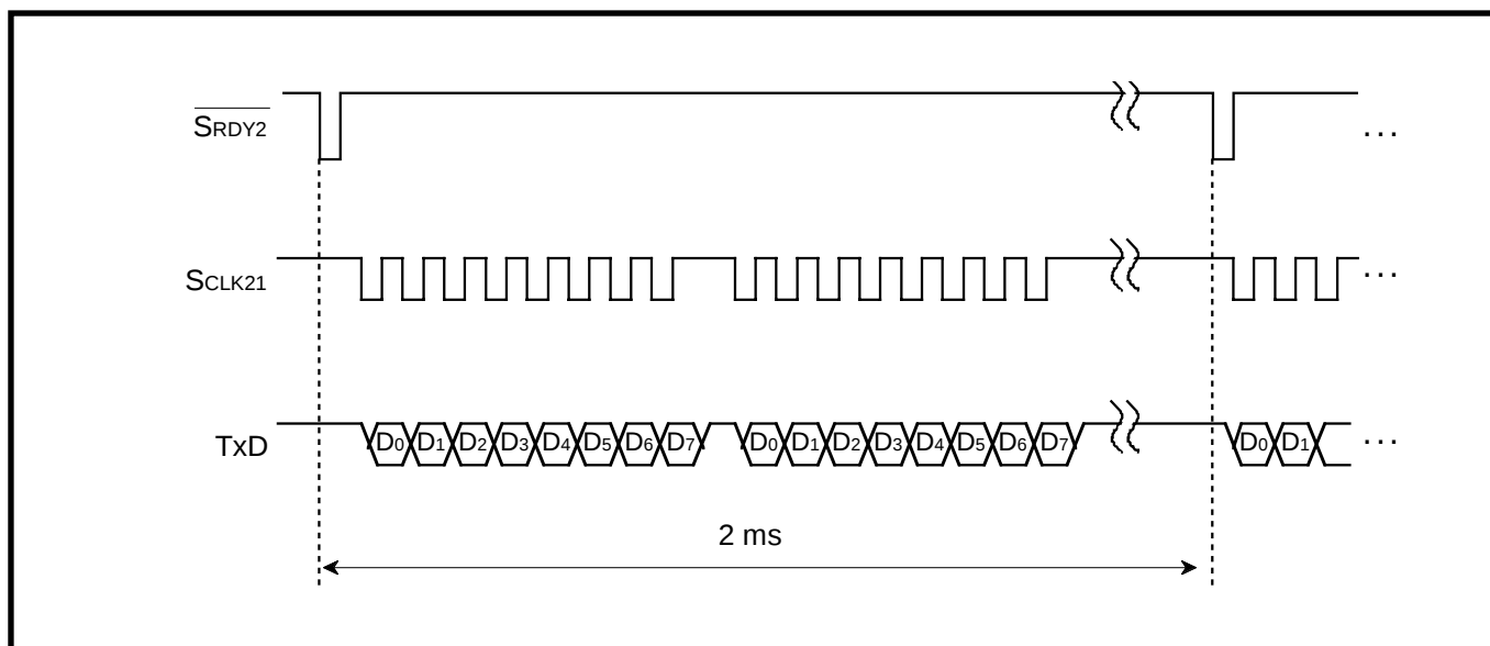
Fig. 2.3.34 Timing chart
