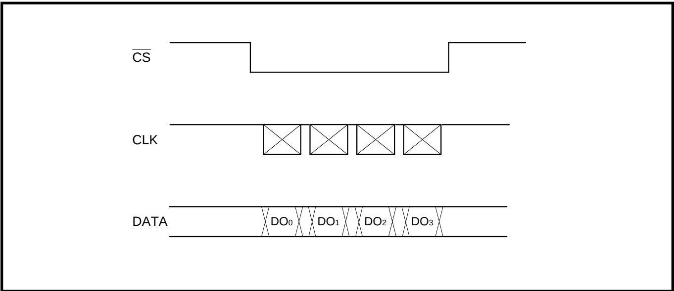
Fig. 2.3.21 Timing chart
