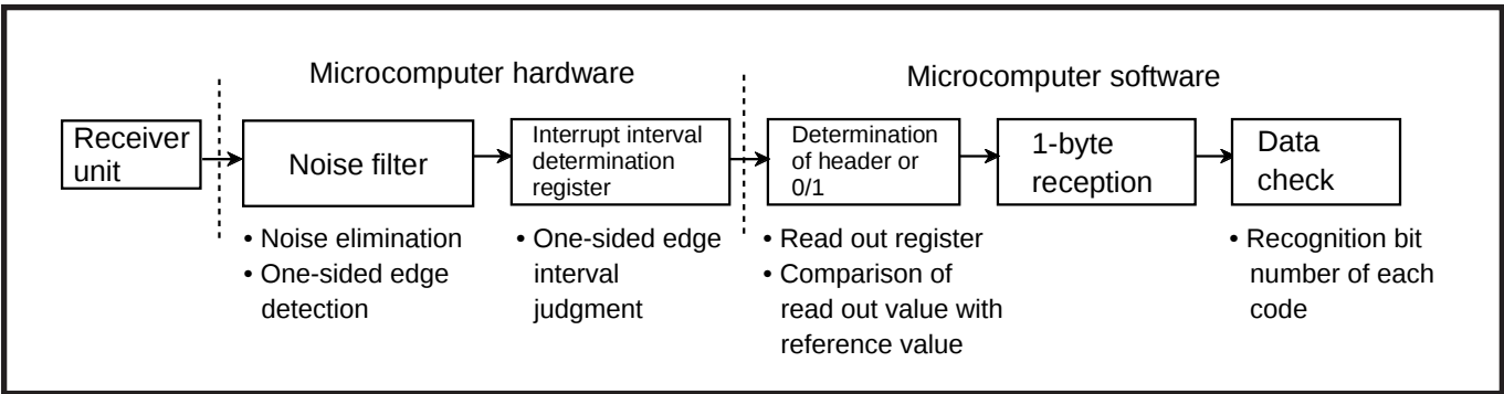
Fig. 2.7.8 Function block diagram
