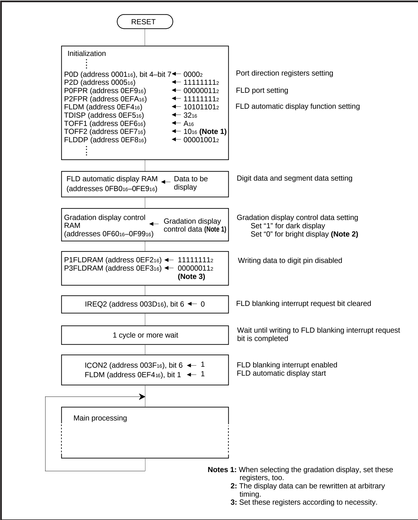
Fig. 2.4.20 Control procedure
