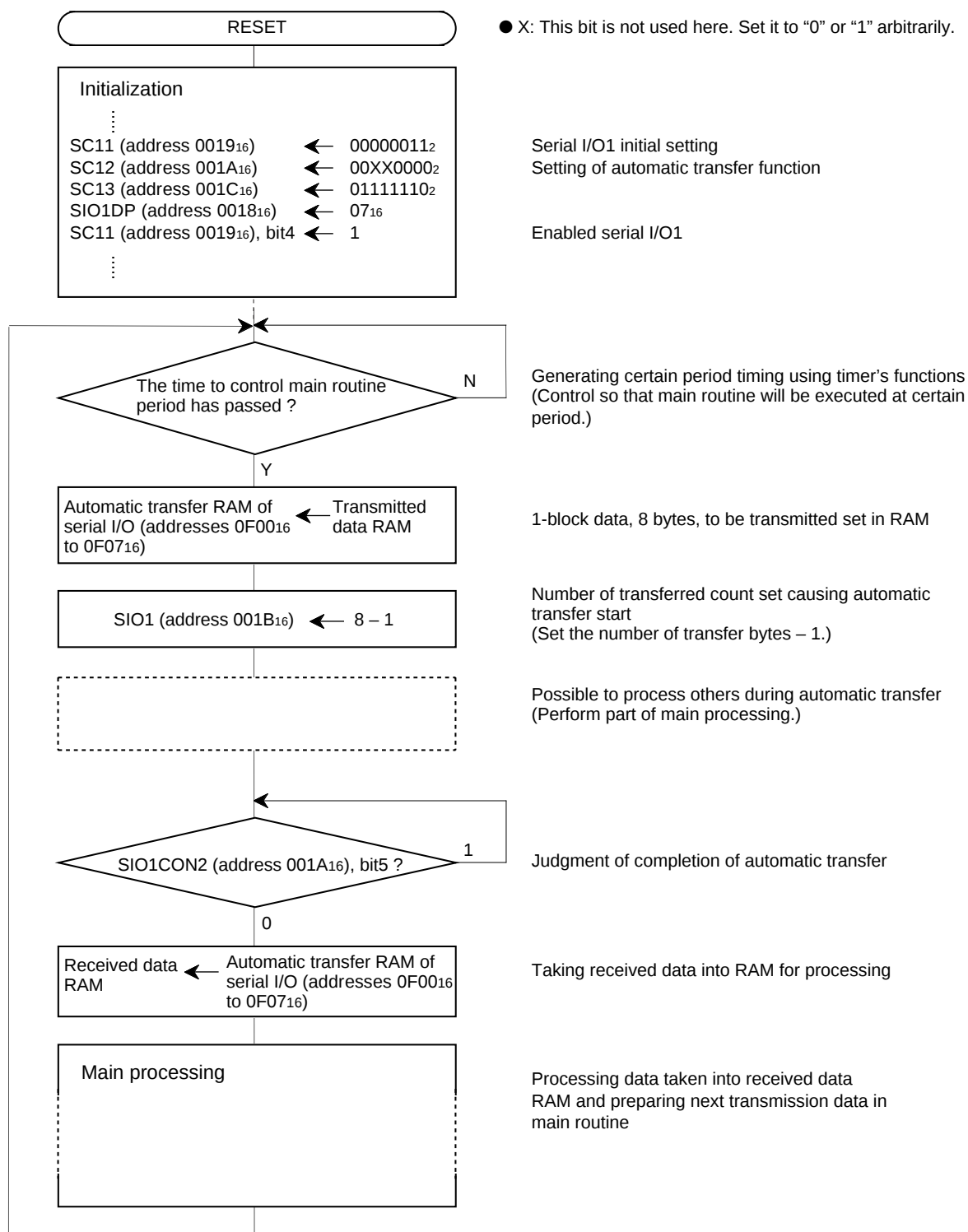
Fig. 2.3.28 Control procedure
