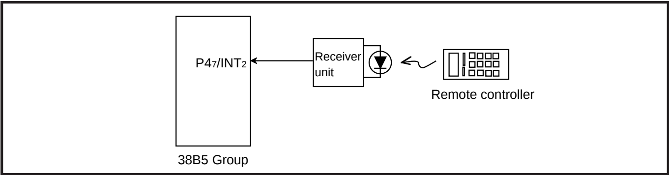
Fig. 2.7.7 Connection diagram
