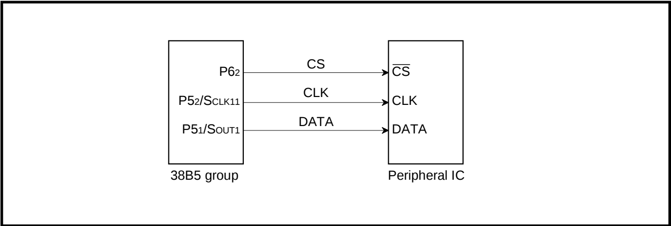
Fig. 2.3.20 Connection diagram
