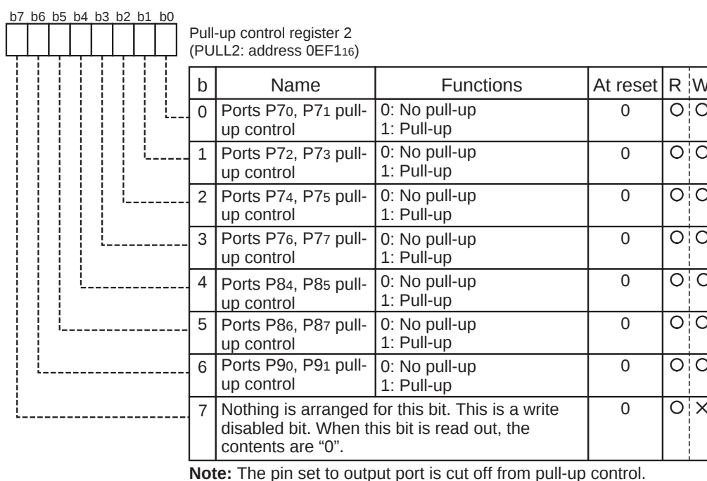
Fig. 3.5.43 Structure of pull-up control register 2
