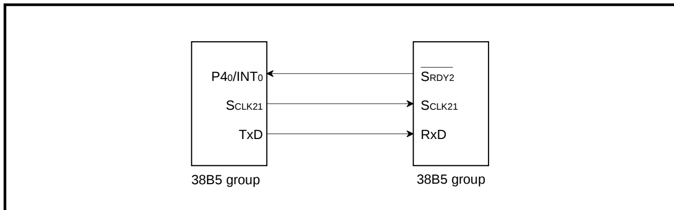
Fig. 2.3.33 Connection diagram
