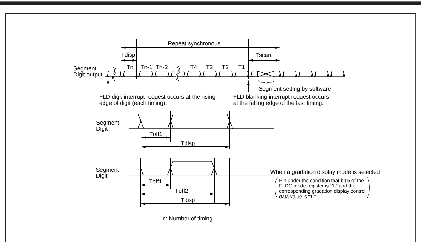
Fig. 51 FLDC timing
