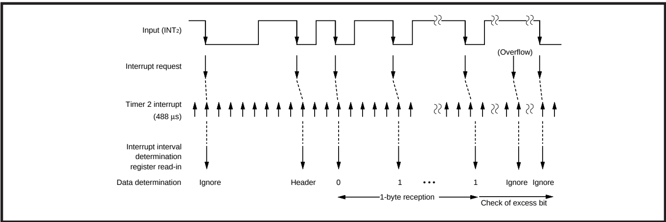
Fig. 2.7.9 Timing chart of data determination
