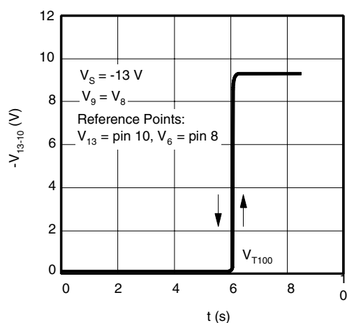
Figure 14. Overload Switching
