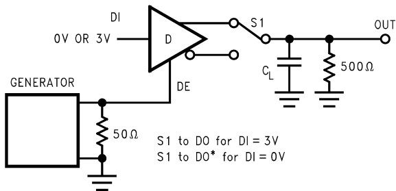
FIGURE 7. TRI-STATE and Sleep Mode Test Circuit ( t_{PZH} , ( t_{PSH} ), t_{PHZ} )
