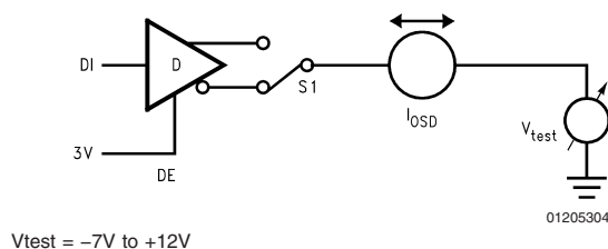
FIGURE 4. Driver I_{ODS}
