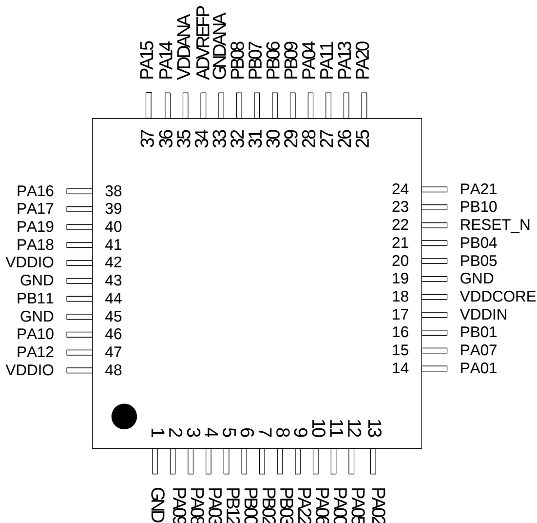
Figure 3-2. TLLGA48 Pinout
