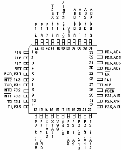
44-Pin QFP
