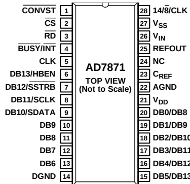
Figure 5. AD7871 DIP
