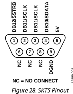
Figure 28. SKT5 Pinout
