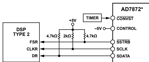
Figure 25. AD7872 to DSP Type 2 Interface
