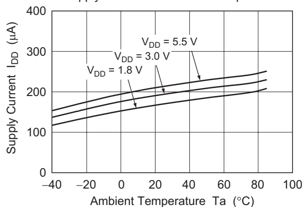
Figure 1-2. HA1630Q04 Supply Current vs. Ambient Temperature
