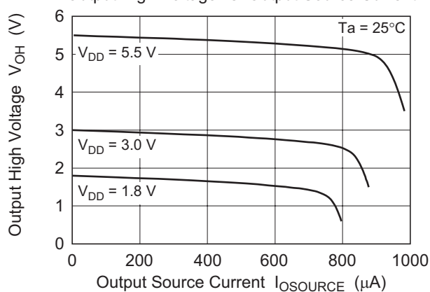
Figure 3-3. HA1630Q06 Output High Voltage vs. Output Source Current
