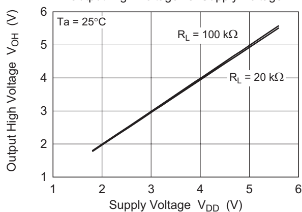
Figure 3-4. HA1630Q06 Output High Voltage vs. Supply Voltage
