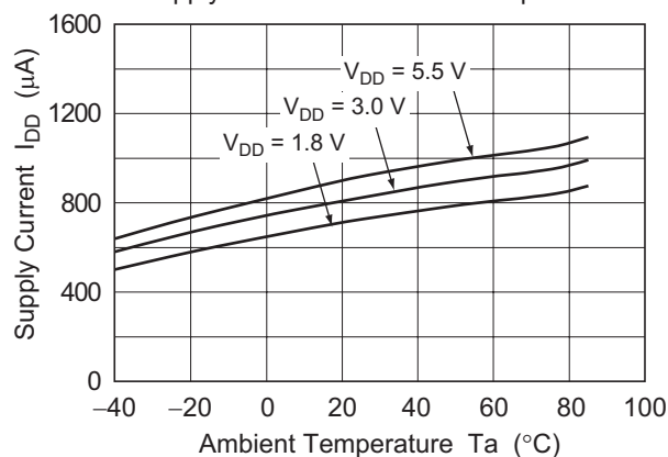
Figure 3-2. HA1630Q06 Supply Current vs. Ambient Temperature
