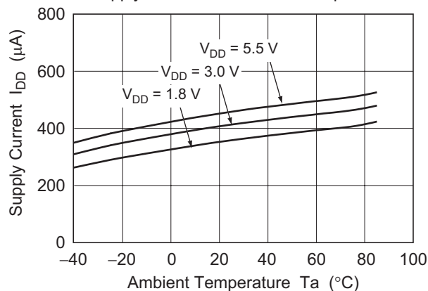
Figure 2-2. HA1630Q05 Supply Current vs. Ambient Temperature
