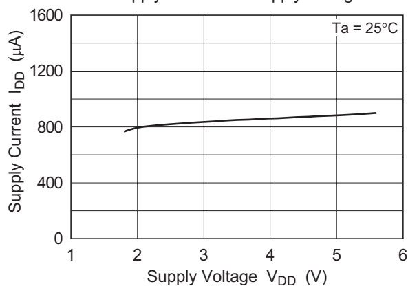
Figure 3-1. HA1630Q06 Supply Current vs. Supply Voltage
