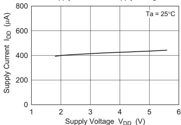
Figure 2-1. HA1630Q05 Supply Current vs. Supply Voltage
