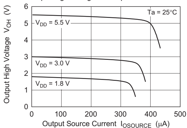
Figure 2-3. HA1630Q05 Output High Voltage vs. Output Source Current
