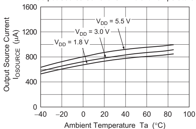
Figure 3-5. HA1630Q06 Output Source Current vs. Ambient Temperature
