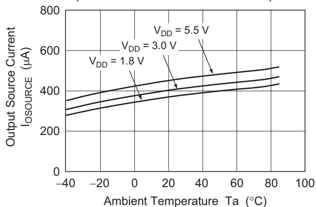
Figure 2-5. HA1630Q05 Output Source Current vs. Ambient Temperature
