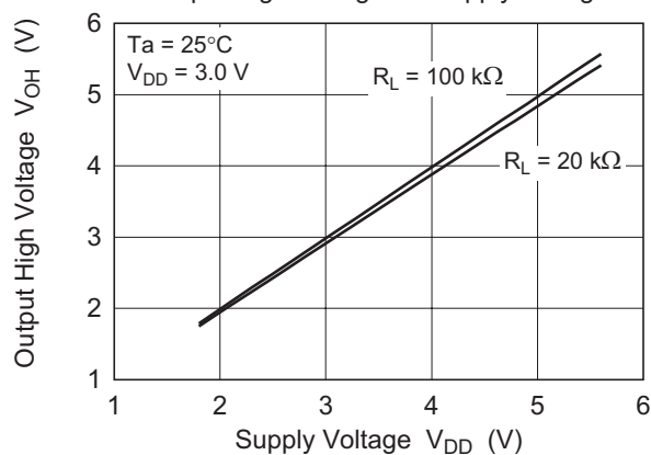
Figure 2-4. HA1630Q05 Output High Voltage vs. Supply Voltage
