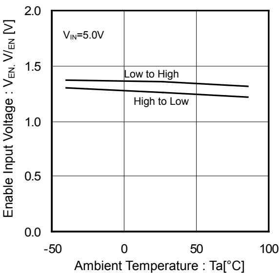
Figure 9. EN, /EN Input Voltage vs Ambient Temperature
