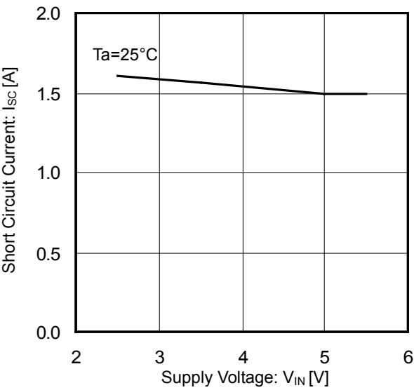
Figure 16. Short Circuit Current vs Supply Voltage
