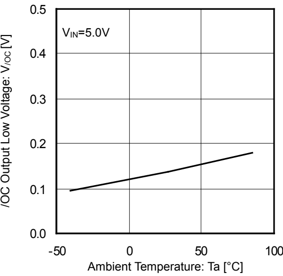
Figure 11. /OC Output Low Voltage vs Ambient Temperature
