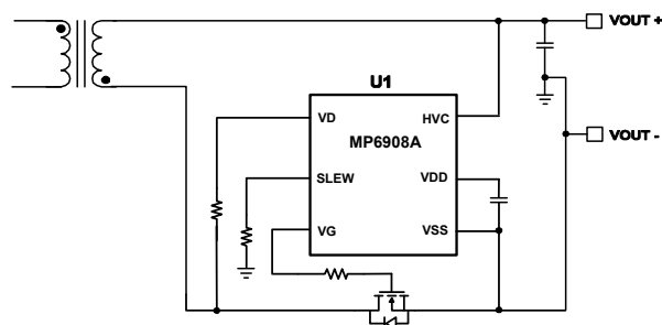
Figure 5: Low-Side Rectification
