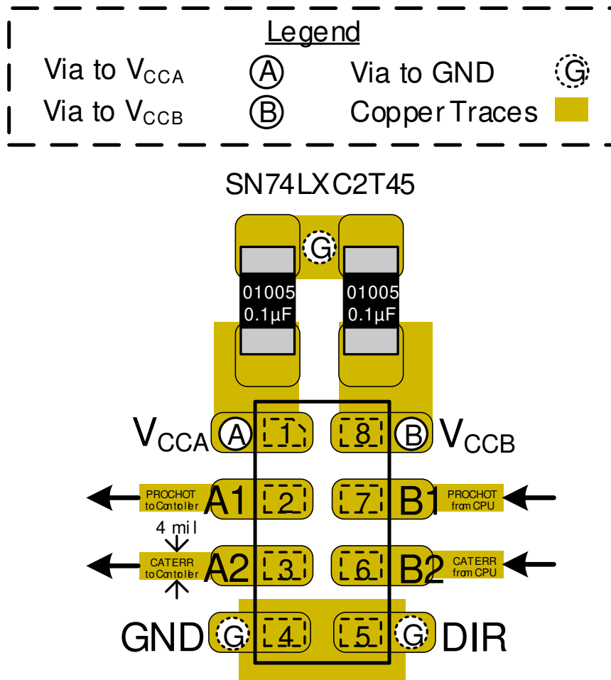
Figure 11-1. Layout Example—SN74LXC2T45DTT
