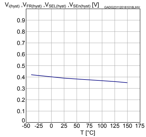
Figure 21. Logic input hysteresis voltage
