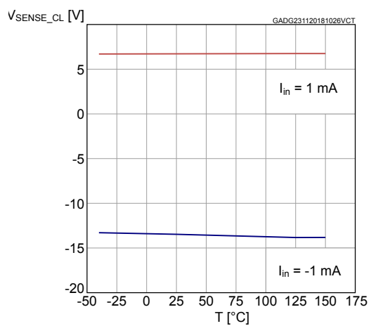
Figure 32. V_{\text{SENSE\_CL}} vs. T_{\text{case}}
