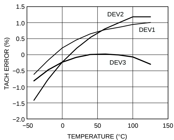
Figure 18. TACH Accuracy vs. Temperature
