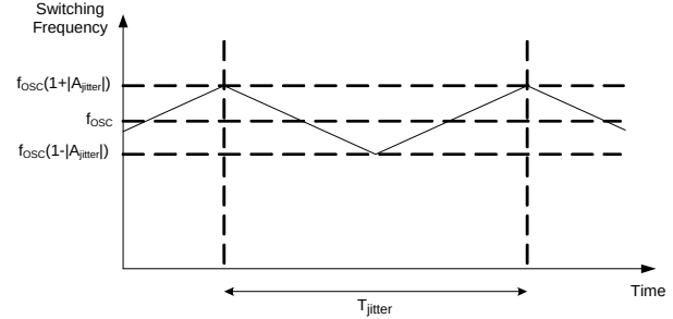
Figure 3: Frequency Jittering
