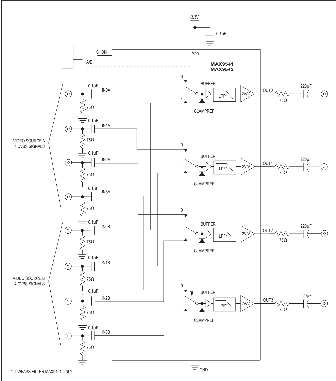
Figure 3. AC-Coupled Outputs
