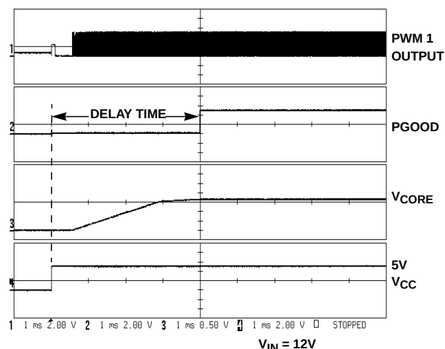
FIGURE 3. START-UP OF A SYSTEM OPERATING AT 500kHz
