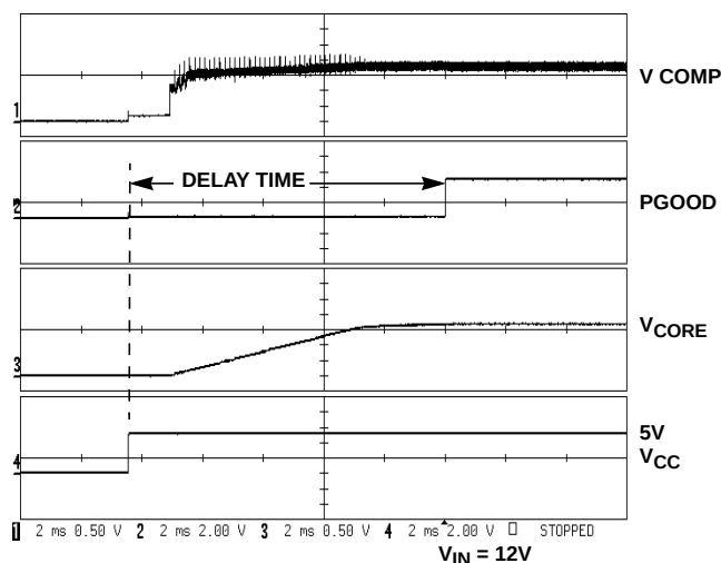
FIGURE 4. START-UP A SYSTEM OPERATING AT 200kHz
