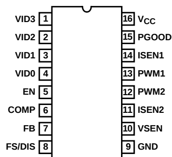
HIP6304 (SOIC) TOP VIEW
