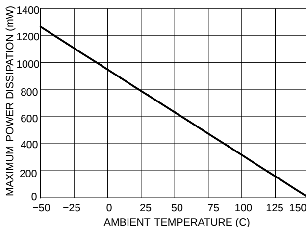
Figure 3. Power Dissipation vs. Temperature
