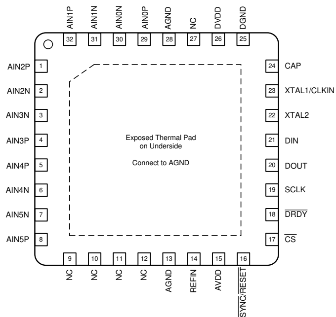
Figure 5-2. RSN Package, 32-Pin WQFN, Top View
