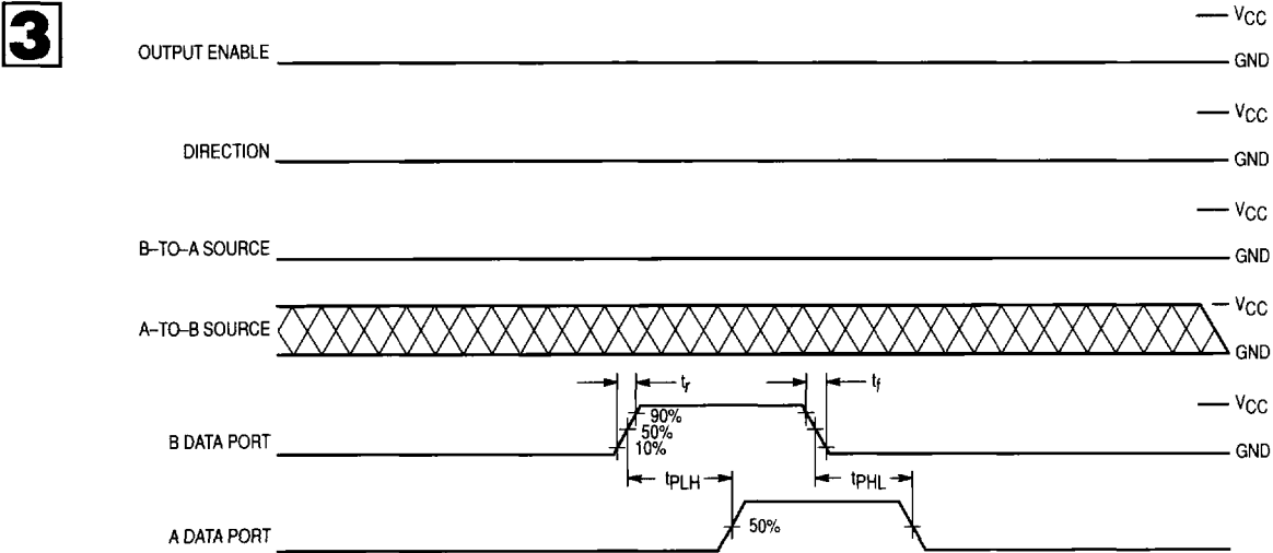
Figure 2. A Data Port = Output, B Data Port = Input
