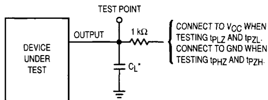
Figure 10. Test Circuit
