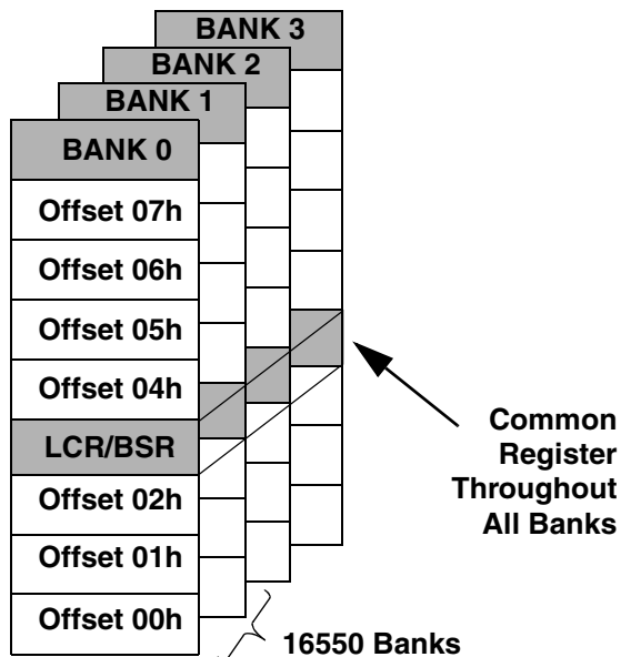
Figure 13. Register Bank Architecture
