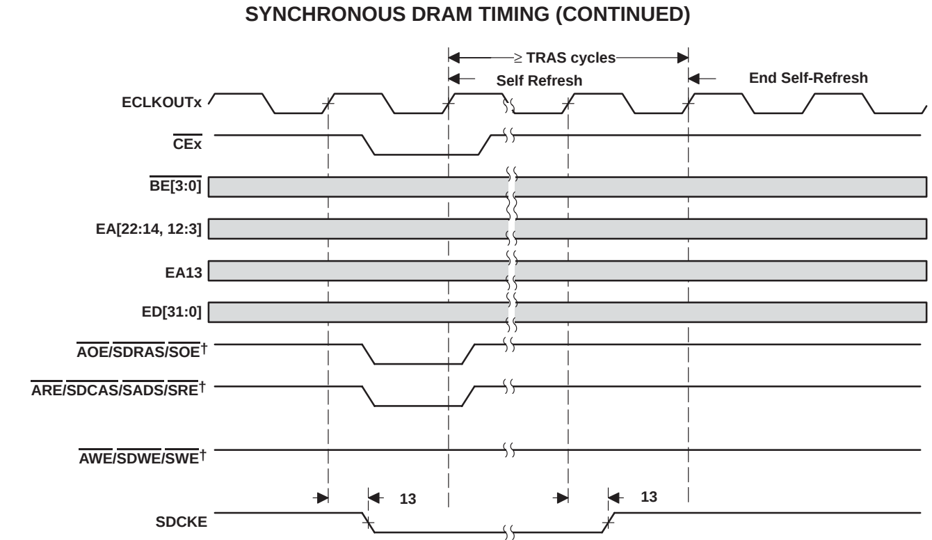
Figure 34. SDRAM Self-Refresh Timing
