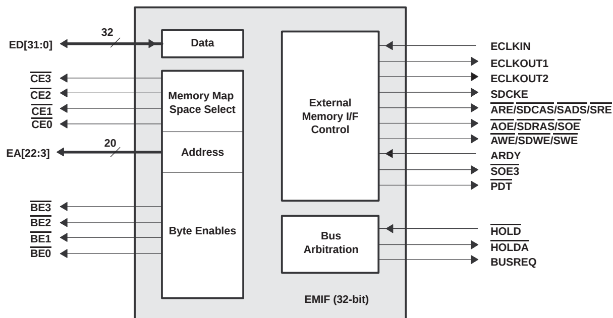
Figure 4. Peripheral Signals
