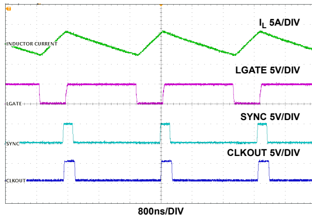
Figure 27. Frequency Synchronization; V_{IN} = 48V , Load = 0A, Default f_{SW} = 300kHz , SYNC f_{SW} = 400kHz
