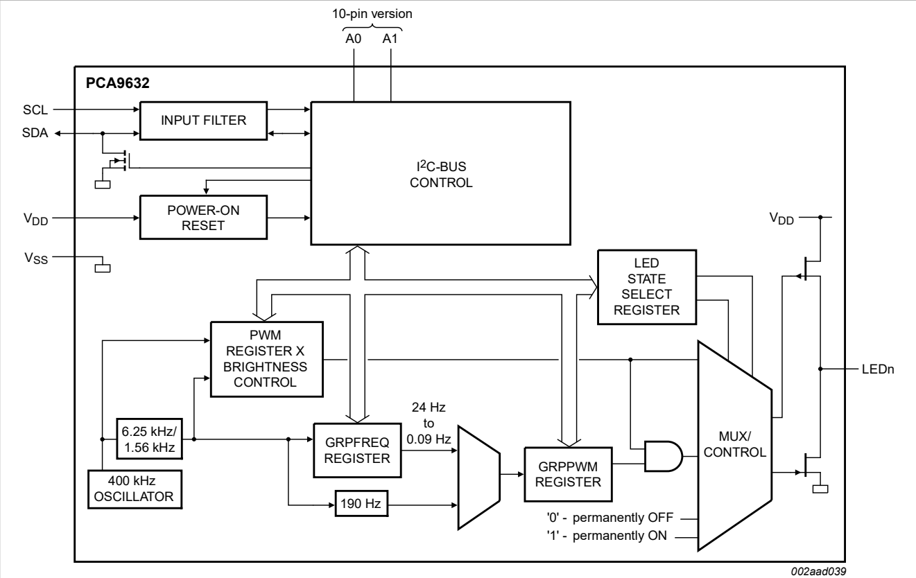
Figure 1. Block diagram of PCA9632
