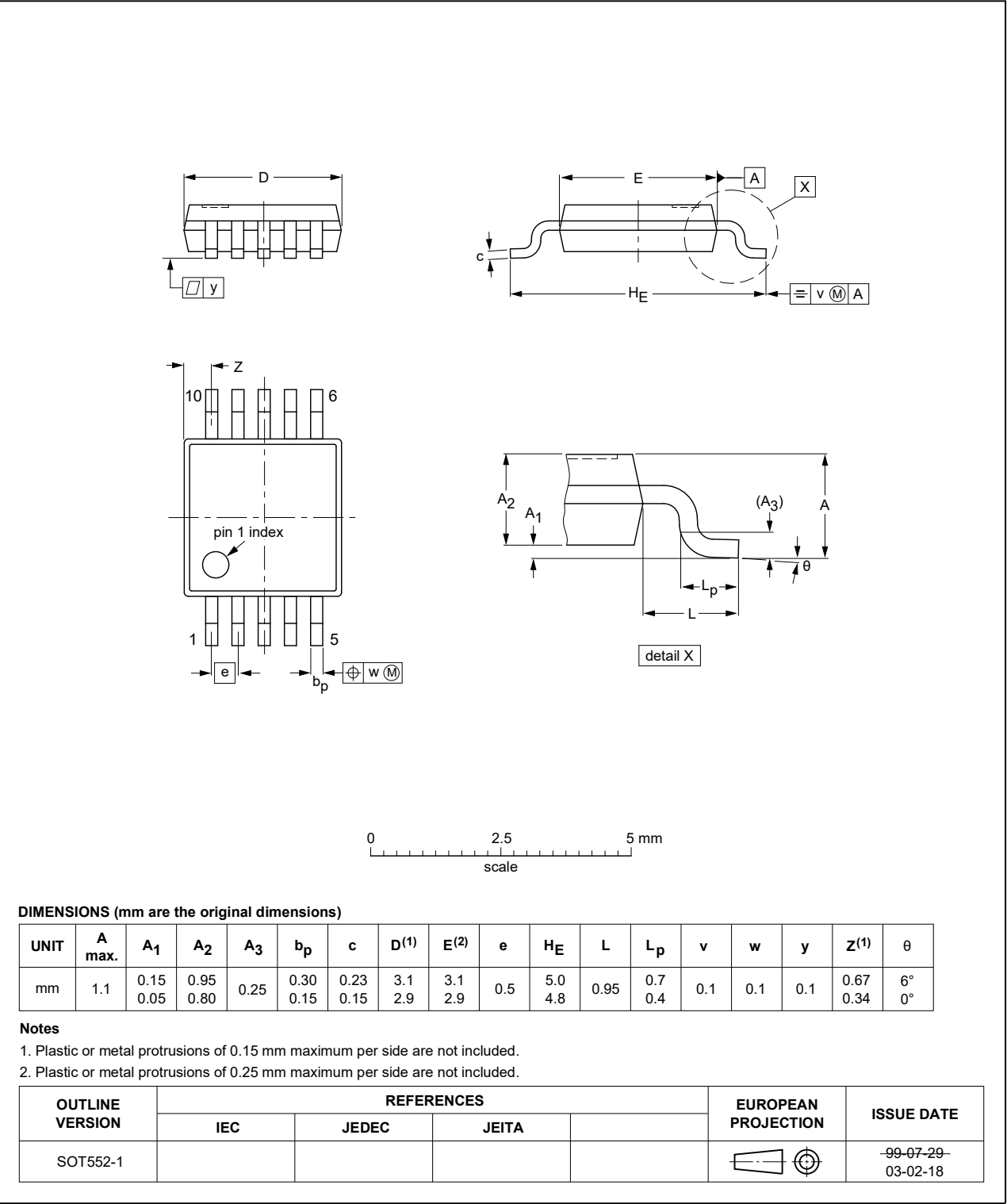
Figure 26. Package outline SOT552-1 (TSSOP10)
