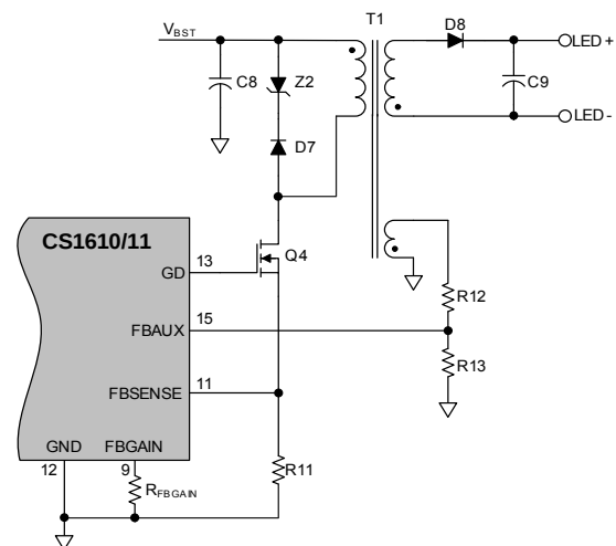
Figure 12. Flyback Model
