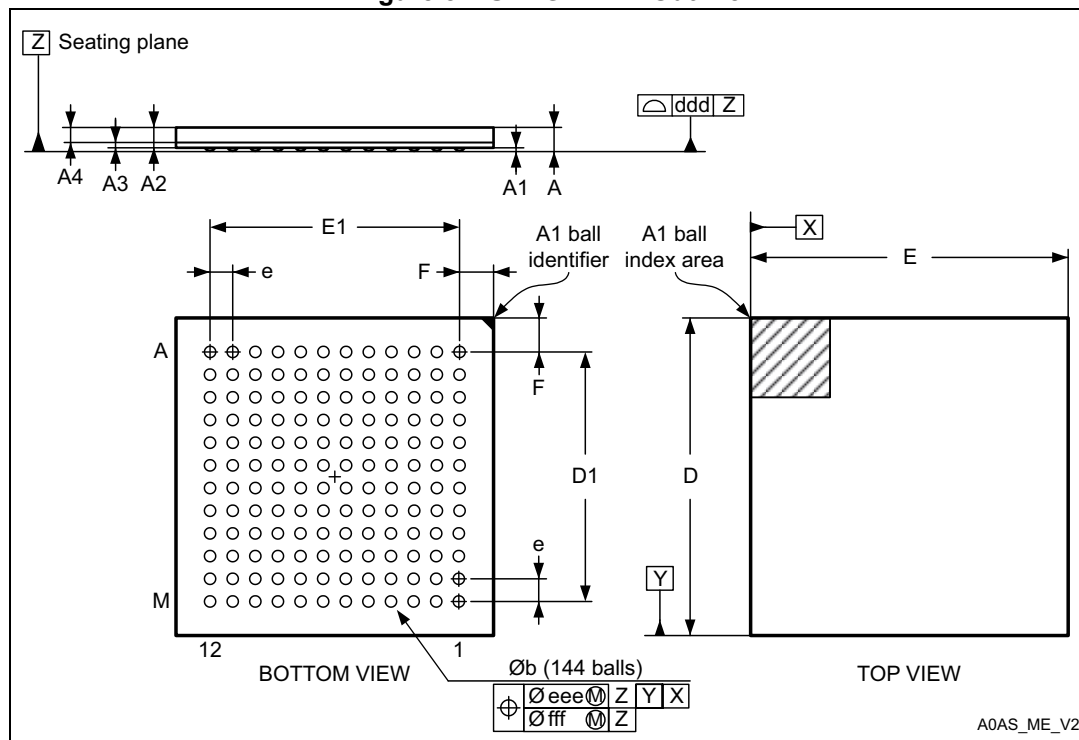
Figure 81. UFBGA144 - Outline
