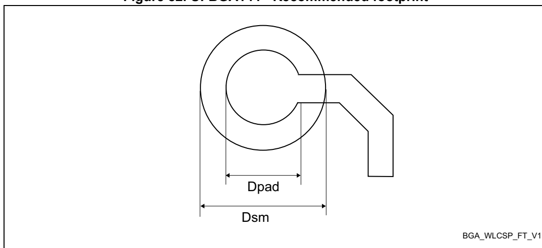
Figure 82. UFBGA144 - Recommended footprint
